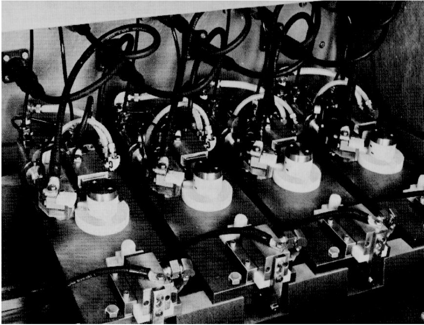
EXAMPLE OF MULTI-TOOLING FOR ELECTRO CHEMICAL DEBURRING OF CONNECTING RODS
