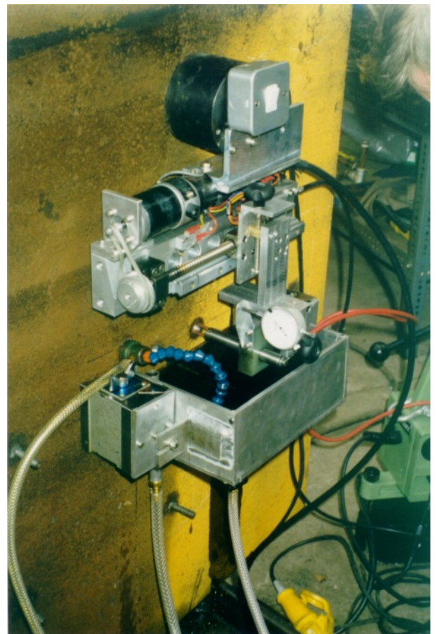
Portable EDM Head & Dielectric Tank held on vessel by Electro-Magnets
