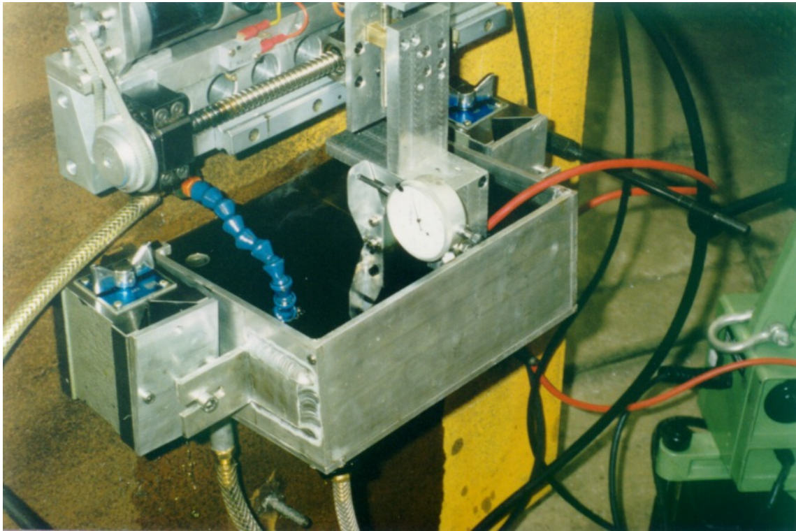
Portable EDM Head & Dielectric Tank held on vessel by Electro-Magnets
